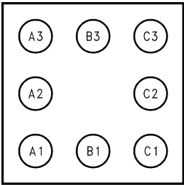
Top View 8 Bump micro SMD Package See NS Package Number BLA08
