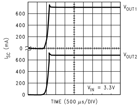
Output Short Circuit Current at V_{IN} = 3.3\text{V}
